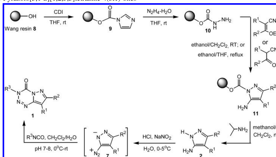
Scheme 2. SPS of Pyrazolo[5,1- d ][1,2,3,5]tetrazine-4(3 H )-ones
